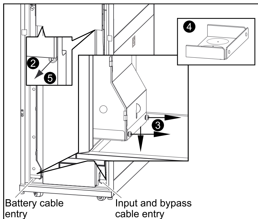
Rear View of the UPS
