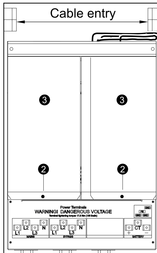
Top View of the Cable Landing Area
